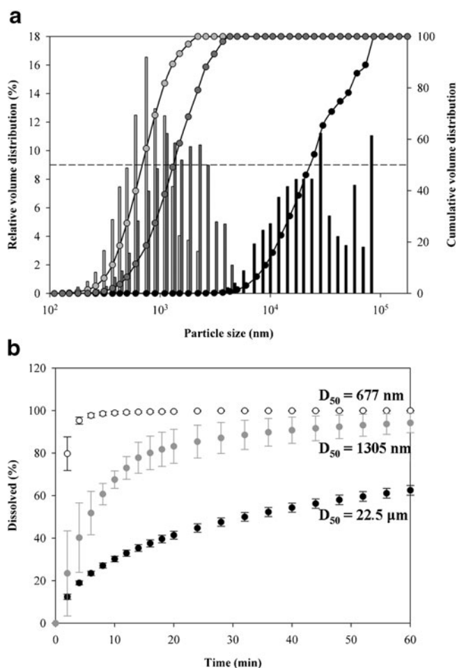
Fig. 5 (a) Particle size distribution of the crystalline dispersions obtained from the 25 mg/mL (light grey) and 50 mg/mL (dark grey) dipyrnidamole in TBA solution and the physical mixture (black). (b) Dissolution profiles of dipyrnidamole from tablets composed of the physical mixture (filled circle) and controlled crystallized dispersions. The dispersions were prepared from a solution containing 25 mg/mL (white circle) and 50 mg/mL (filled circle) dipyrnidamole in TBA. The D_{50} -values in the figure are the values as determined in (a). All tablets contained 10% w/w dipyrnidamole ( n = 3-6 ; mean \pm standard deviation).
